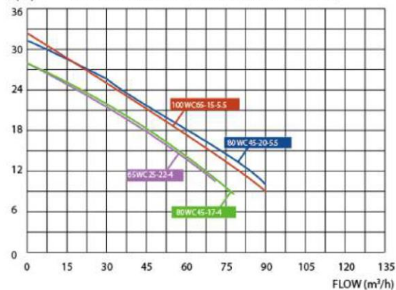
Performance Table (4kw-7.5kw)
